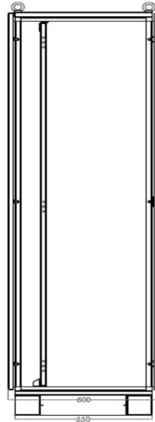
Side View (Without Side Panels)
